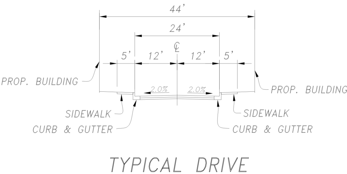
Figure 2-8, Internal Street – No Parking
