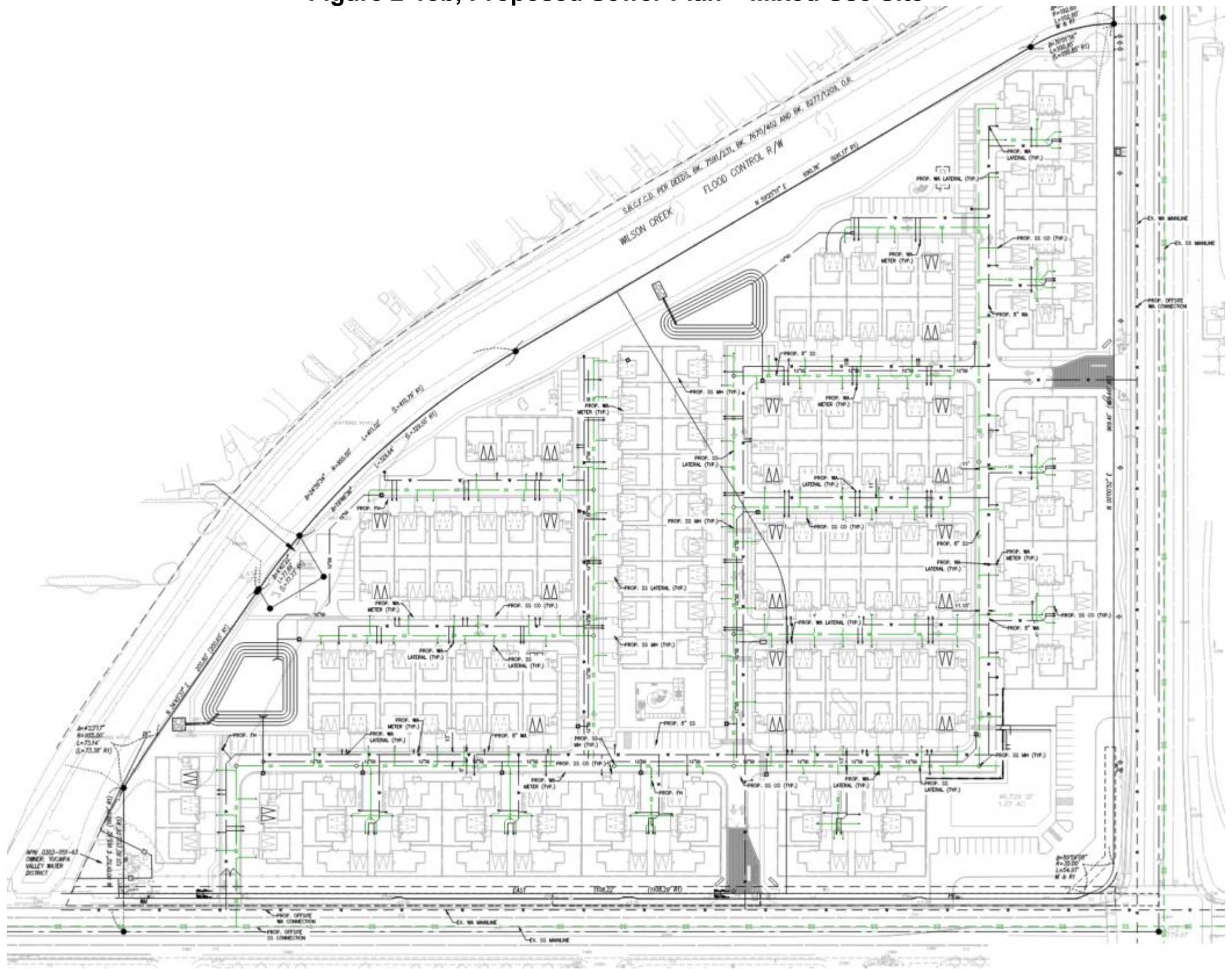
Figure 2-18b, Proposed Sewer Plan – Mixed Use Site
