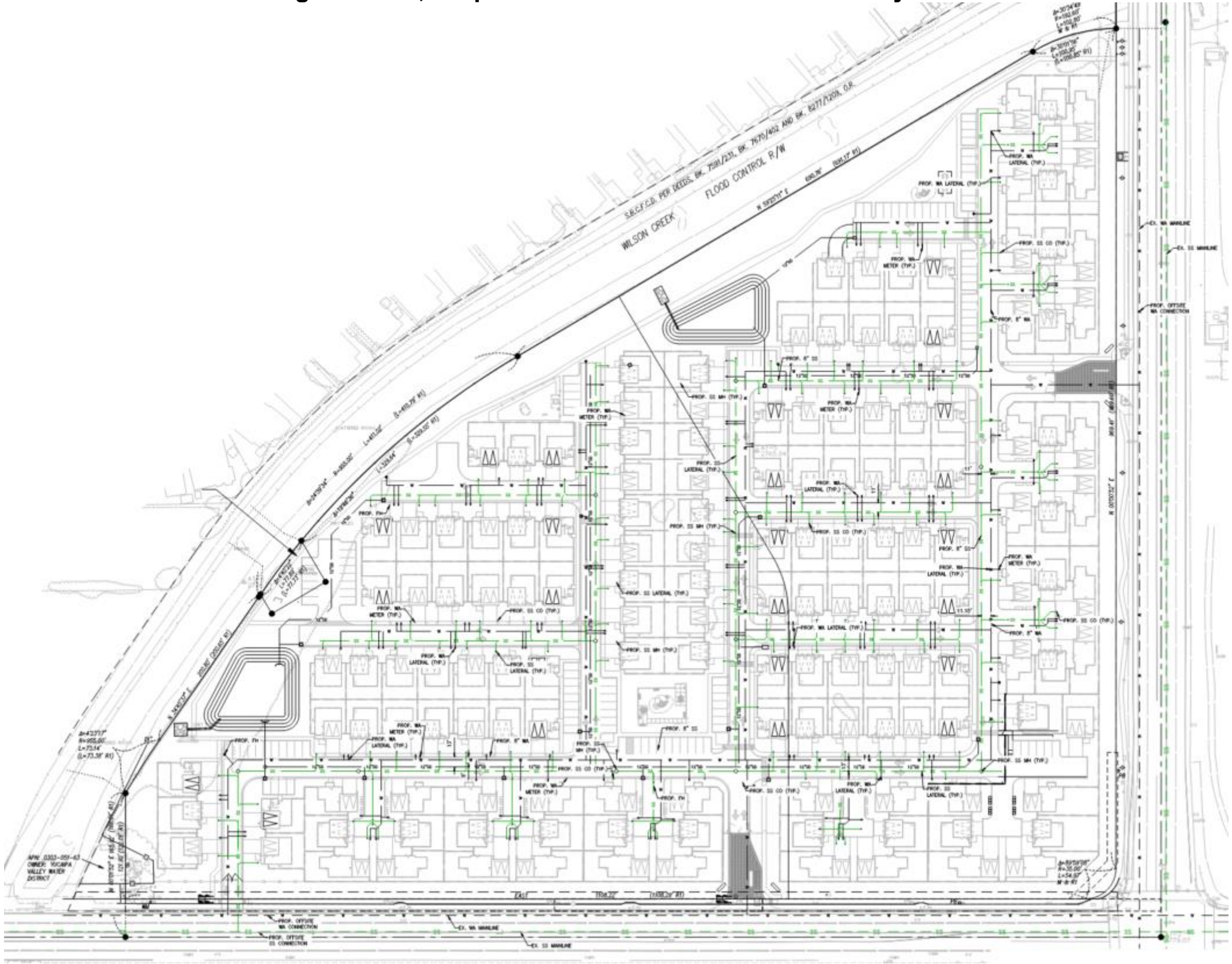
Figure 2-18a, Proposed Sewer Plan – Residential Only Site
