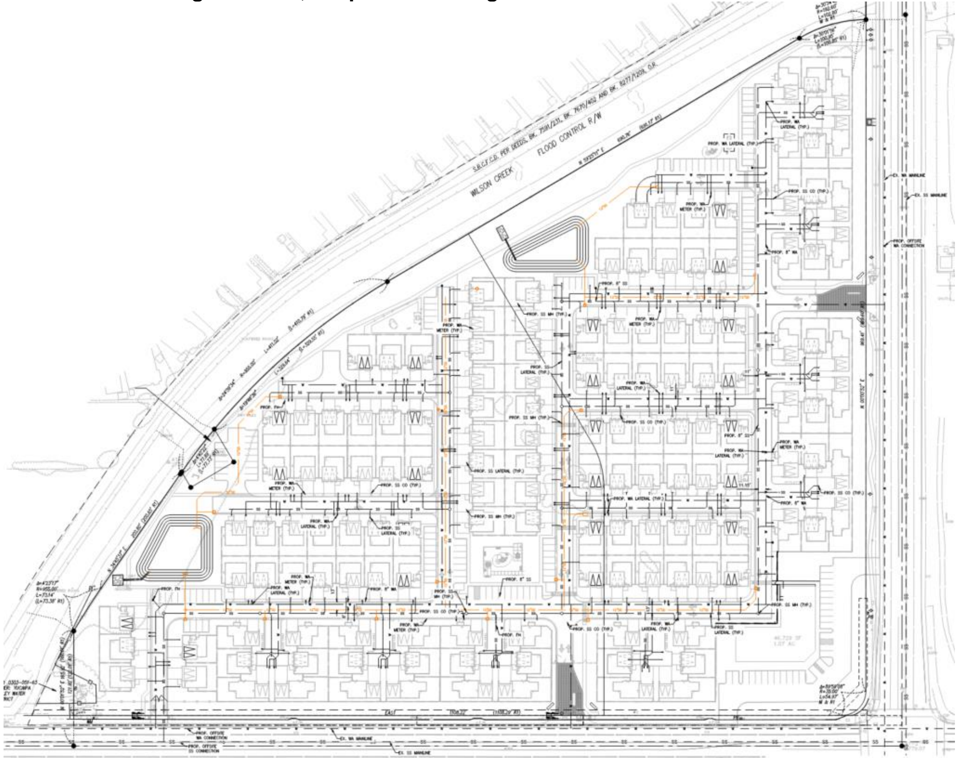
Figure 2-19b, Proposed Drainage Facilities – Mixed Use Site
