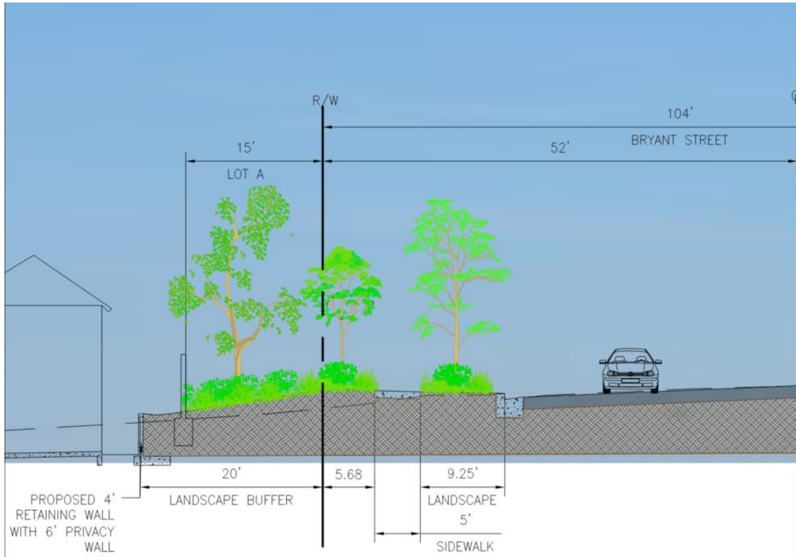
Figure 2-14, East Edge Condition
