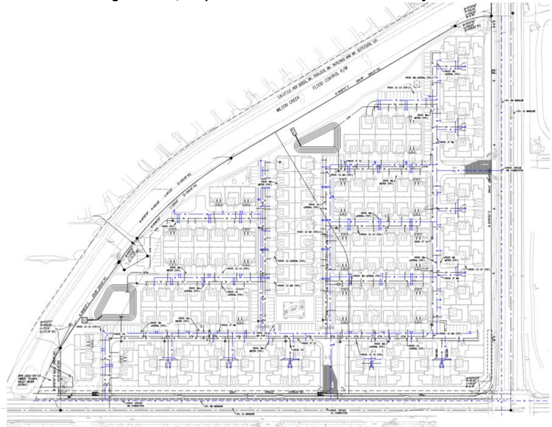
Figure 2-17a, Proposed Water Plan – Residential Only Site
