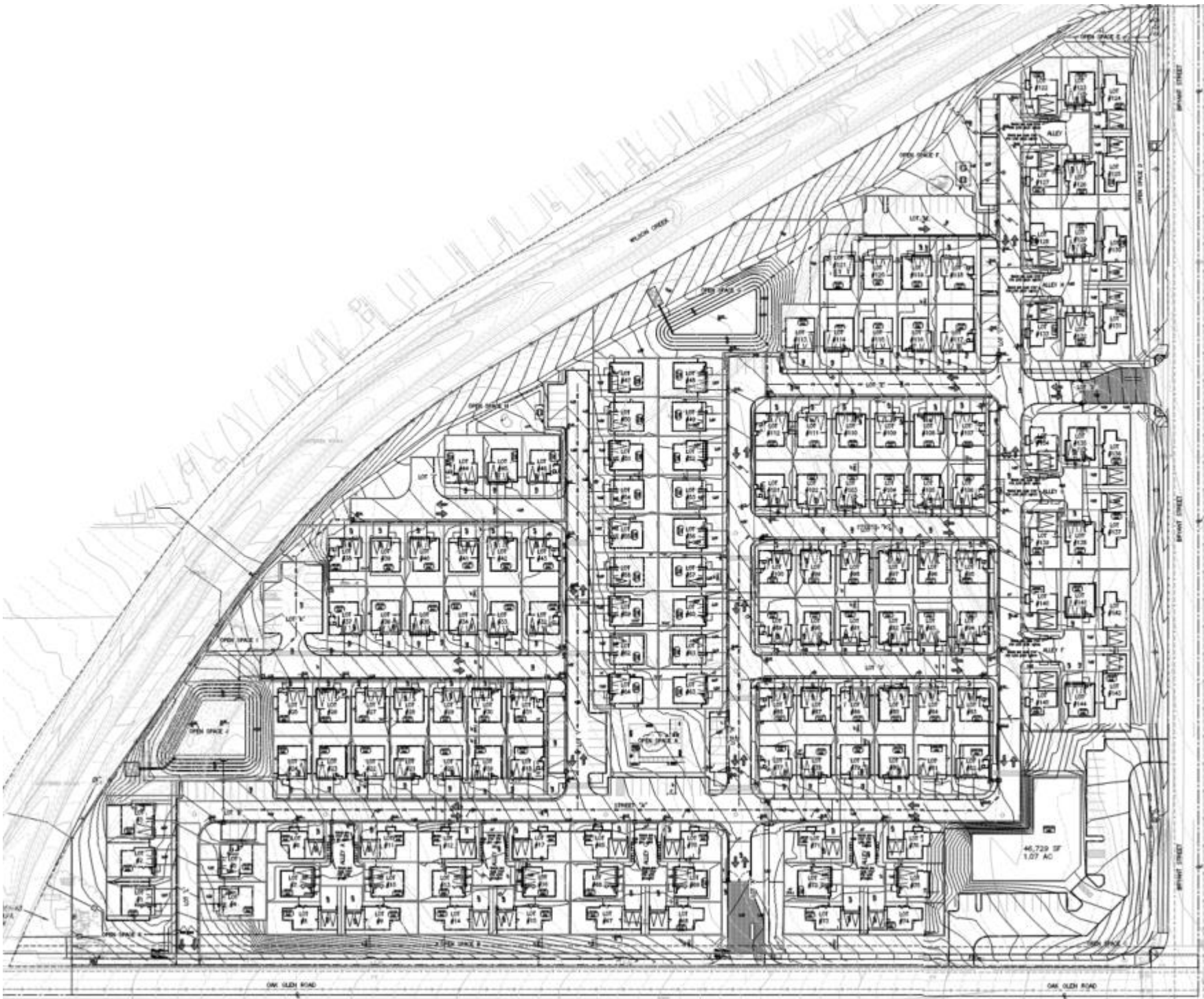
Figure 2-16a, Conceptual Grading – Mixed Used Site
