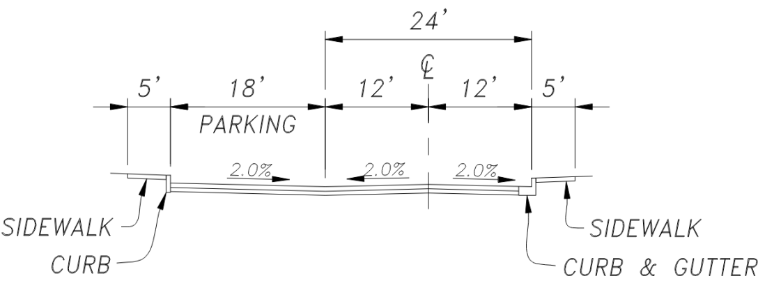
Figure 2-7, Internal Street – Parking 1 Side
